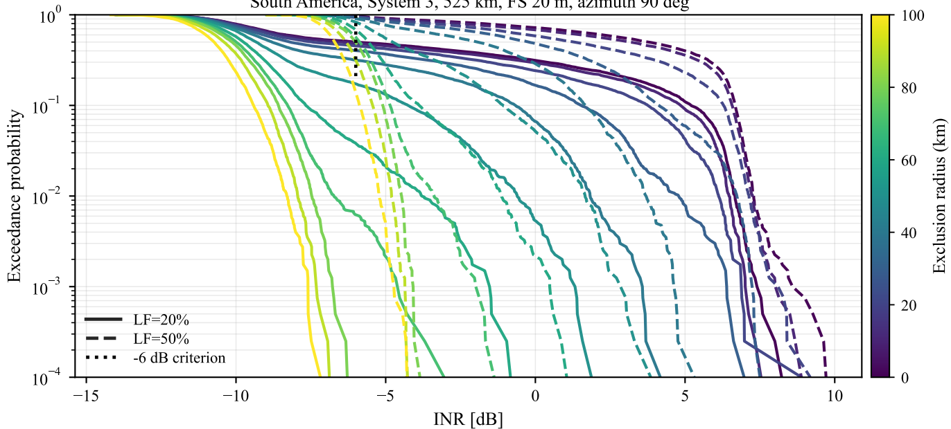
South America, System 3, 525 km, FS 20 m, azimuth 90 deg
